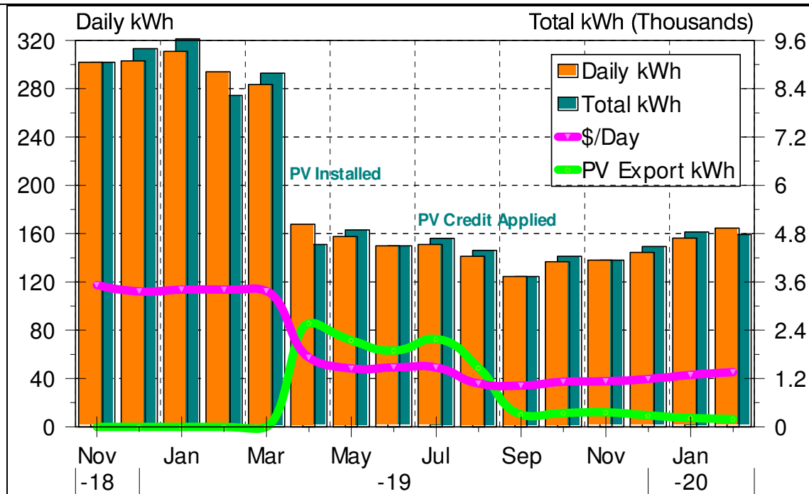
Fig. 5. Electricity Consumption before and after using Solar Energy at Owen's dairy in Oakey.
