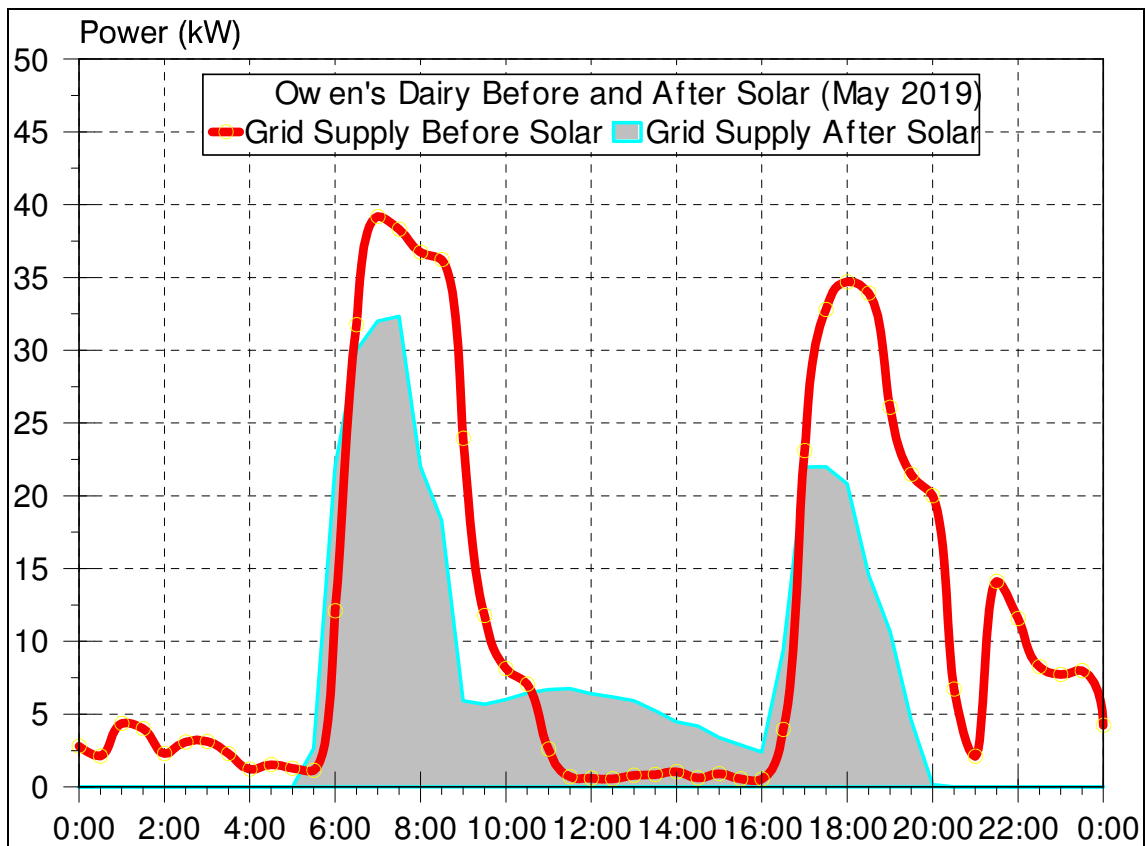
Fig 4. Load curves before and after solar.
