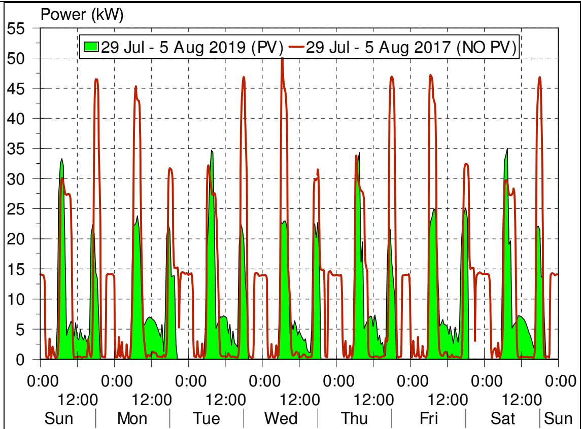
Fig. 3. Consecutive daily load curves before and after solar (green)
